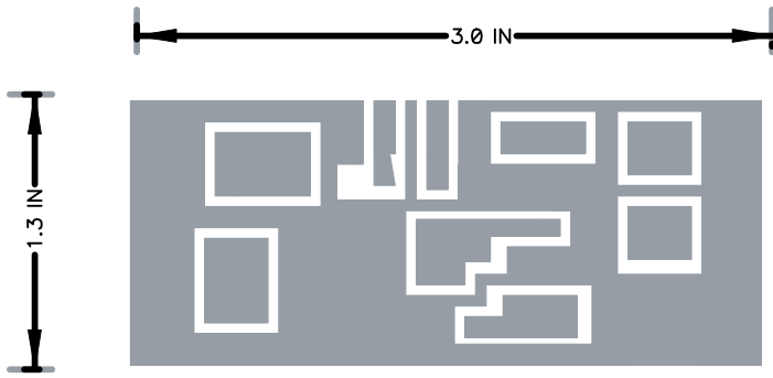
6 Watt Amplifier Board Pattern
