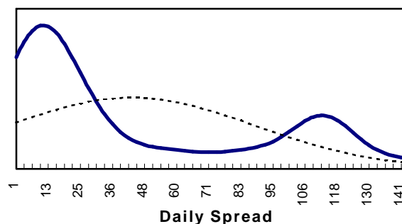
Daily Spread Distribution for Indian Rupee 5/95 - 5/97
