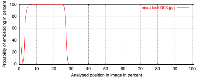
Figure 4: An image containing a message hidden with JSteg shows a high probability of embedding at the beginning of the image. It flattens to zero, when the test reaches the unmodified part of the DCT coefficients.
