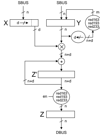
Fig. 6. Shift-and-Add Multiplier. Fig. 7. Least-Significant-Digit-First Multiplier.
