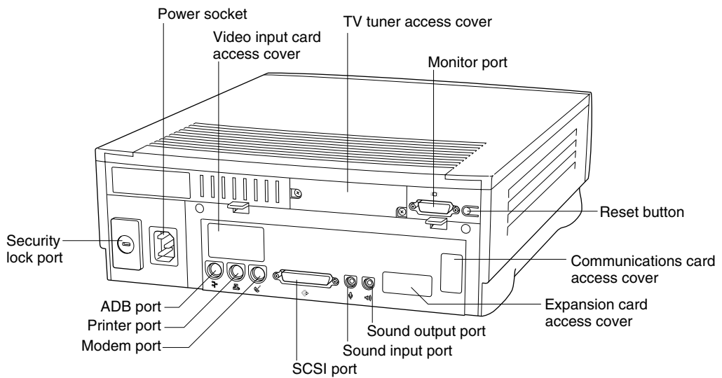
Figure 1-2 Back view of the computer
