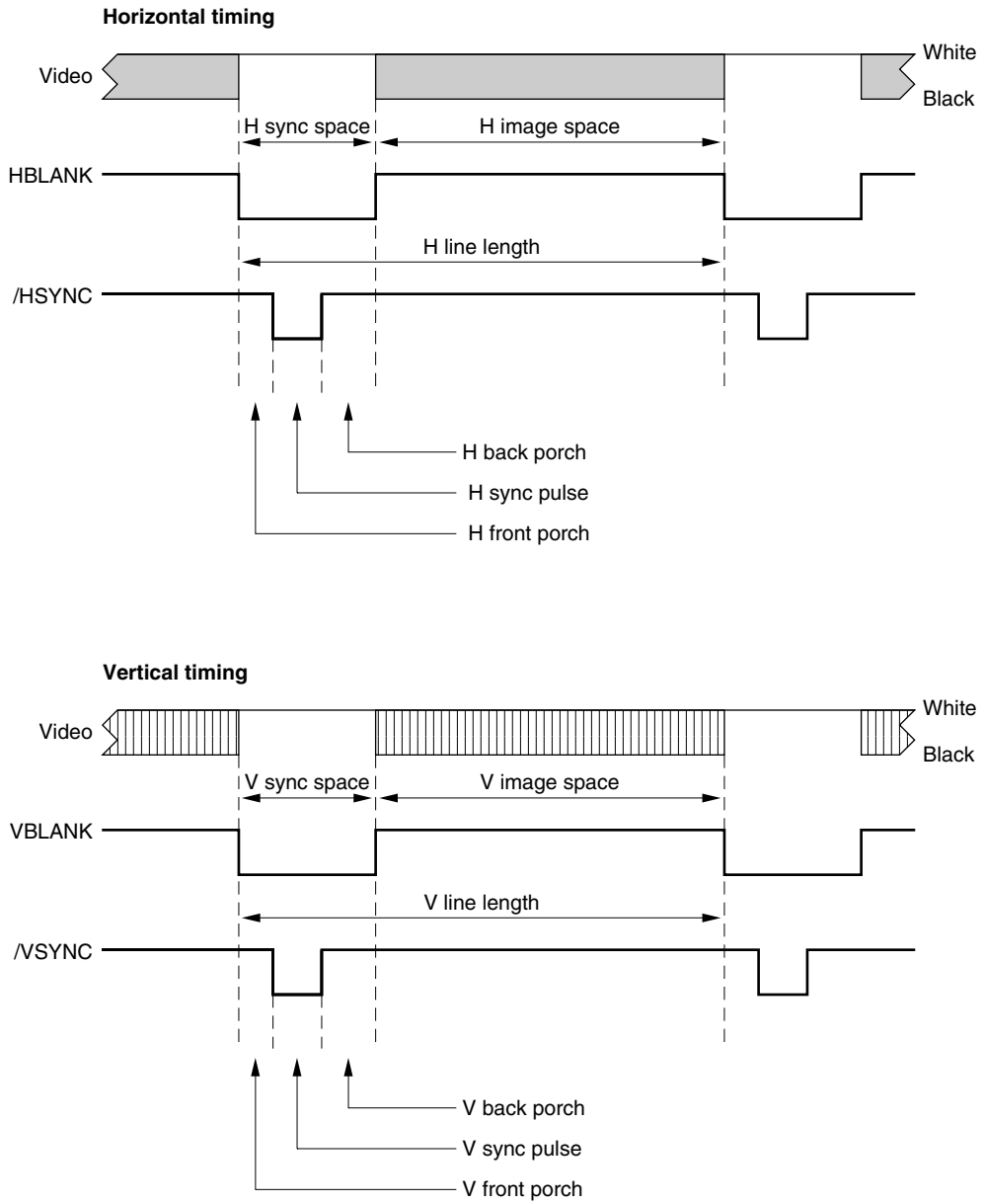
Figure 3-3 Video timing diagram
