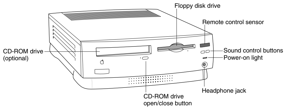
Figure 1-1 Front view of the computer
