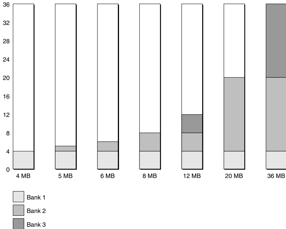
Figure 4-1 RAM configurations
