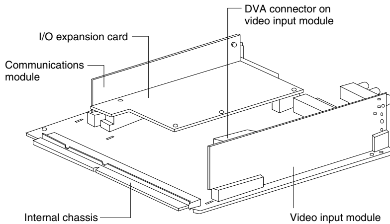
Figure 4-4 Location of the DVA connector
