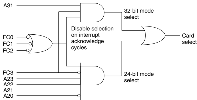
Figure 4-3 Generating the card select signal
