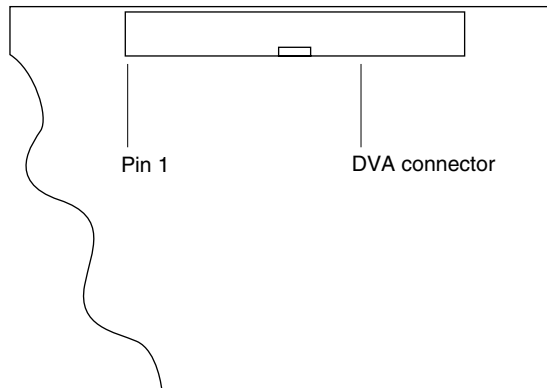
Figure 4-5 Orientation of the DVA connector
