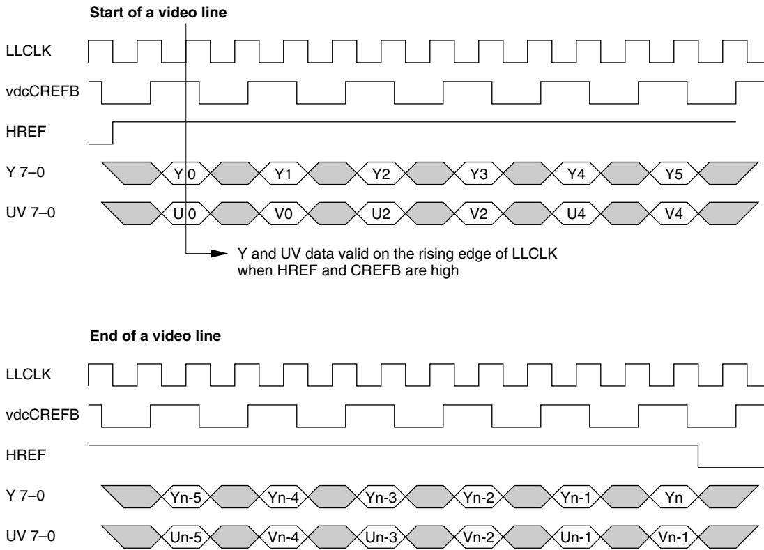
Figure 4-6 Video data timing
