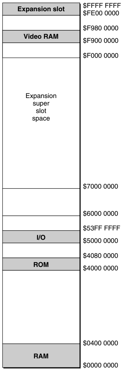
Figure 2-2 Simplified address map
