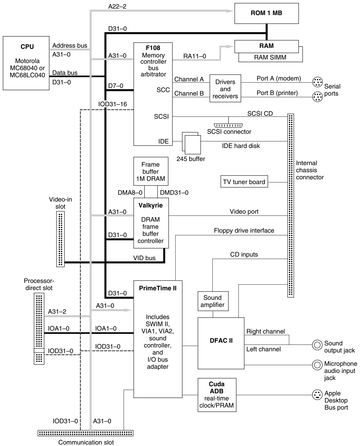
Figure 2-1 Block diagram
