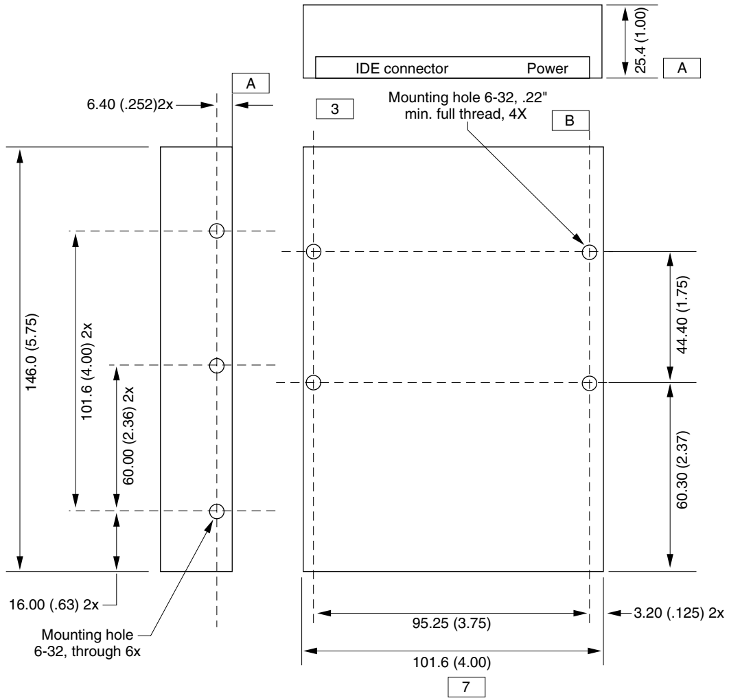
Figure 3-2 Maximum dimensions of the hard disk
