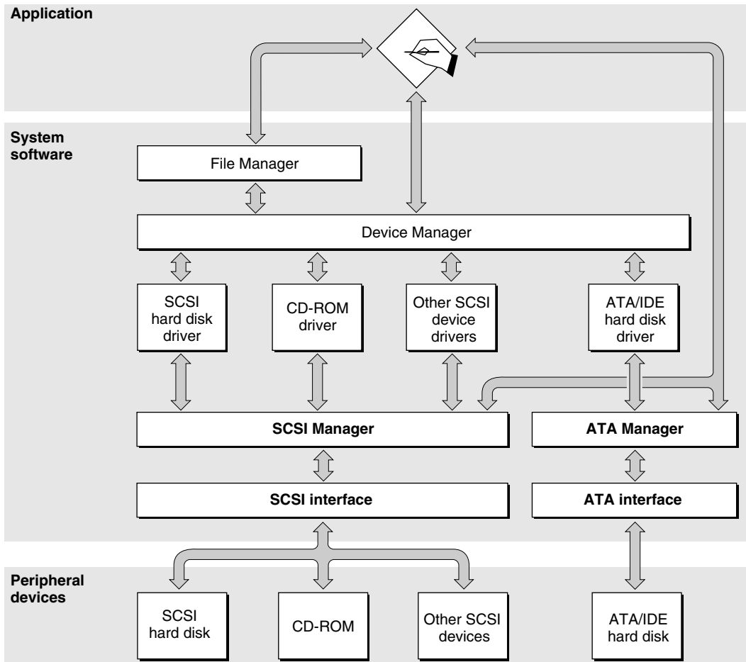
Figure 6-1 Relationship of the ATA Manager to the Macintosh system architecture
