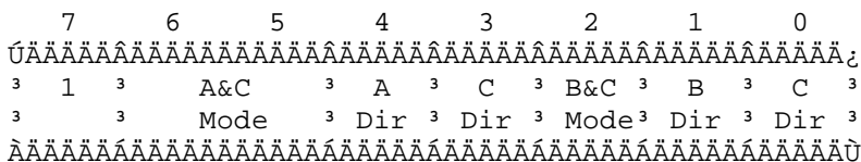
Figure 5: PPI Mode Selection
