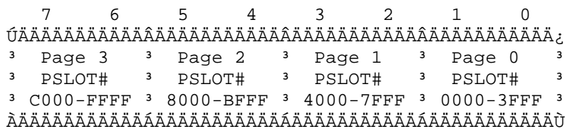
Figure 1: Primary Slot Register
