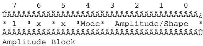
Figure 38: Packet Block Types
